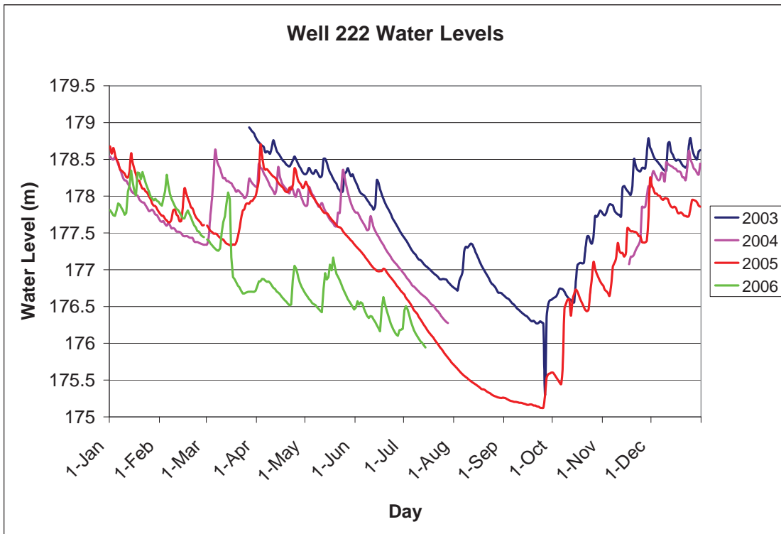
Figure G.2: Well 222 Annual Water Level Comparison
