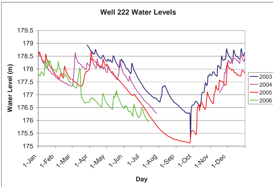
Figure G.2: Well 222 Annual Water Level Comparison
