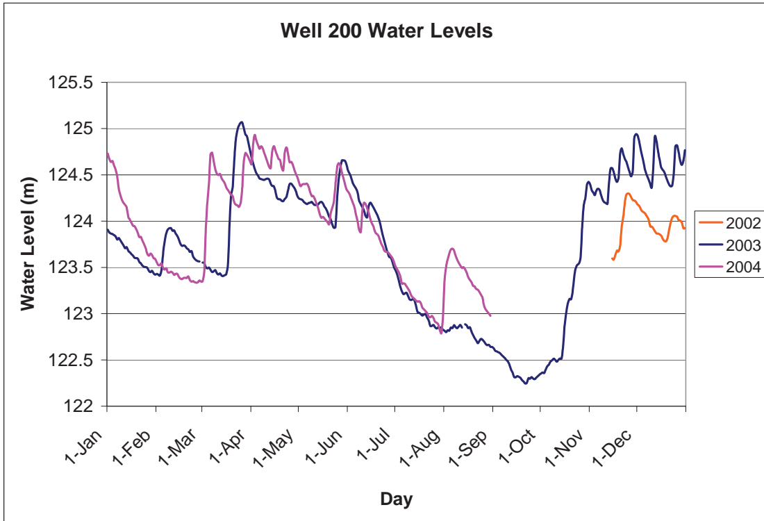
Figure G.1: Well 200 Annual Water Level Comparison
