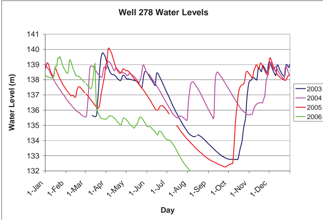
Figure G.3: Well 278 Annual Water Level Comparison
