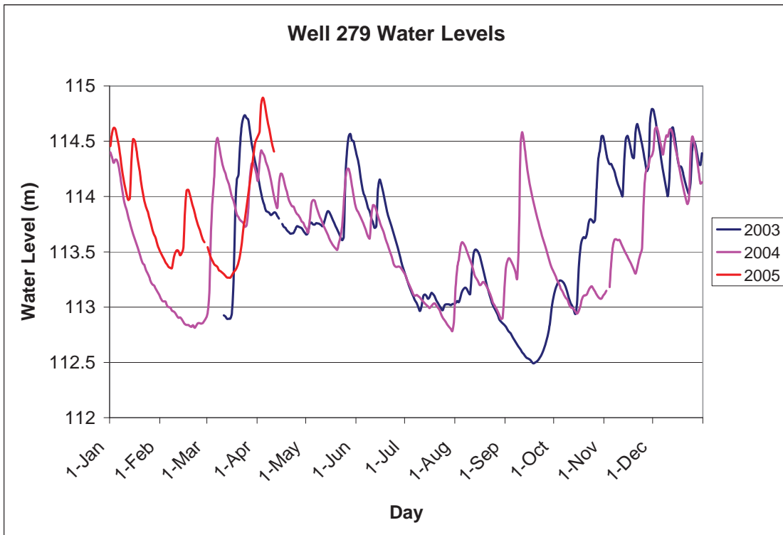
Figure G.4: Well 279 Annual Water Level Comparison
