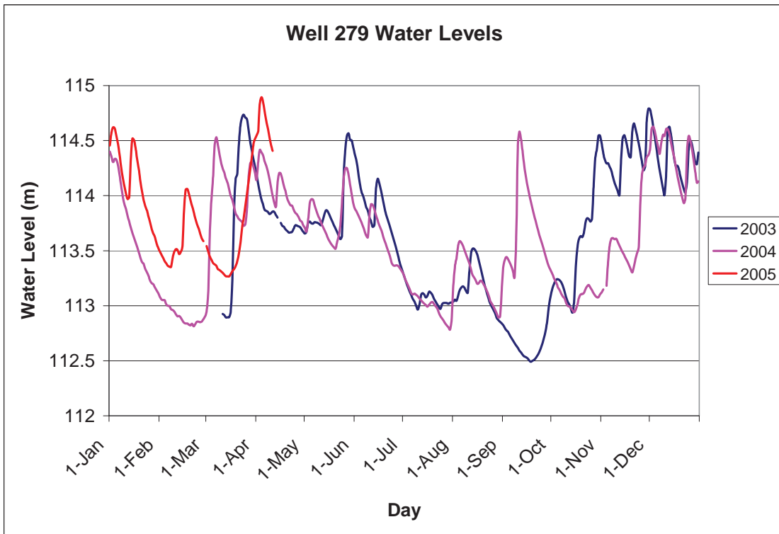
Figure G.4: Well 279 Annual Water Level Comparison
