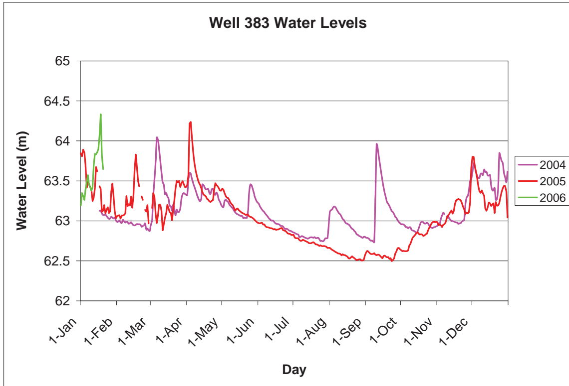
Figure G.7: Well 383 Annual Water Level Comparison
