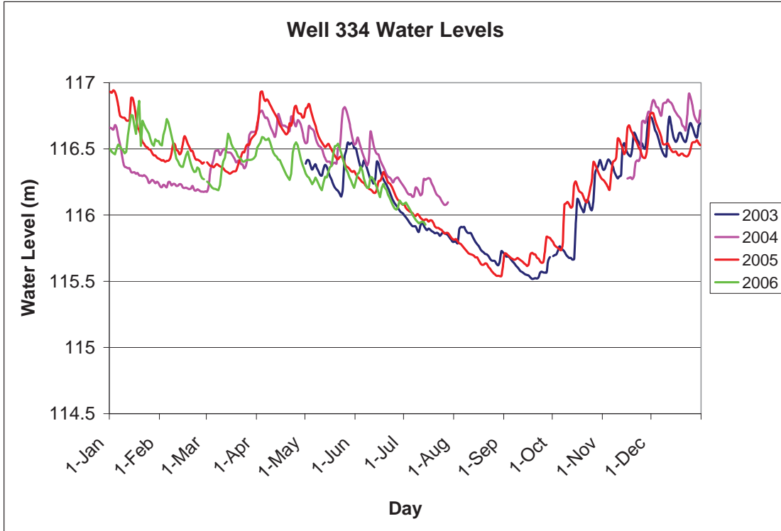
Figure G.5: Well 334 Annual Water Level Comparison
