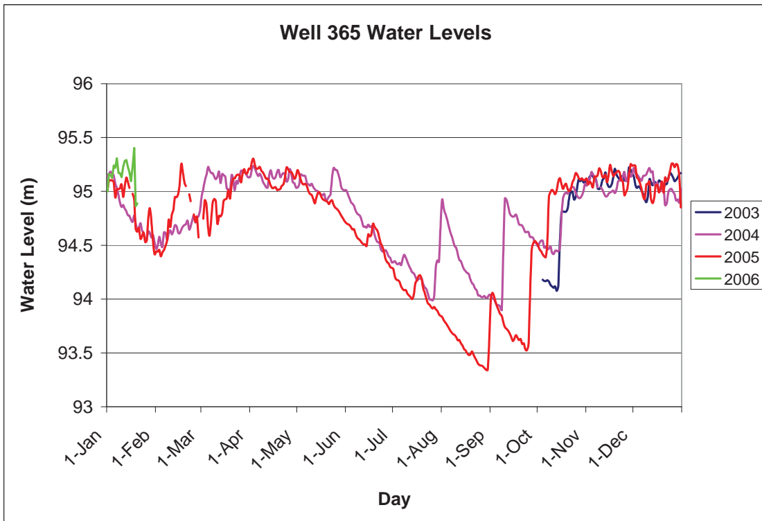
Figure G.6: Well 365 Annual Water Level Comparison
